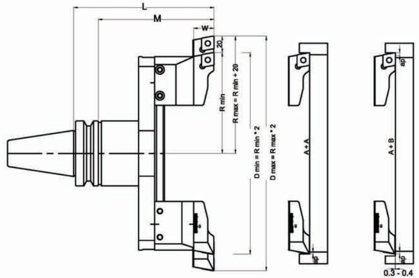
MAS403 BT-B-BIT72 Large Diameter Adjustable Twin Cutter Roughing and Semi-Finishing Boring System
